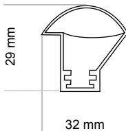
Technical Drawing
